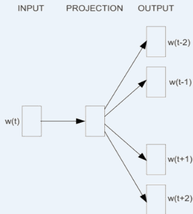
Skip-gram
